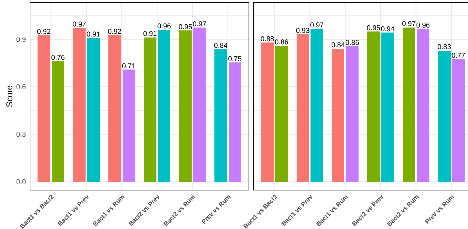
Recall
