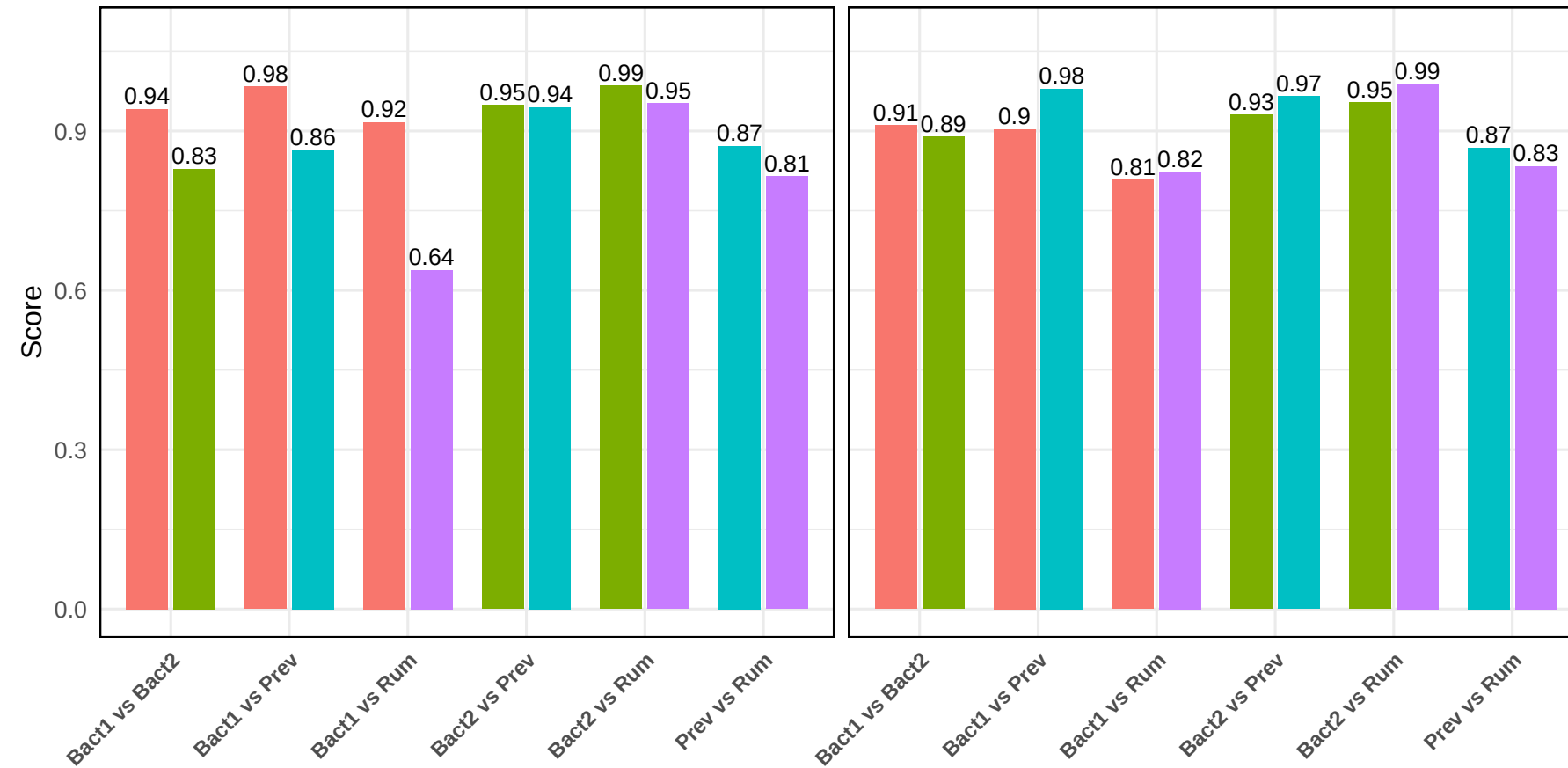
Logistic Regression
