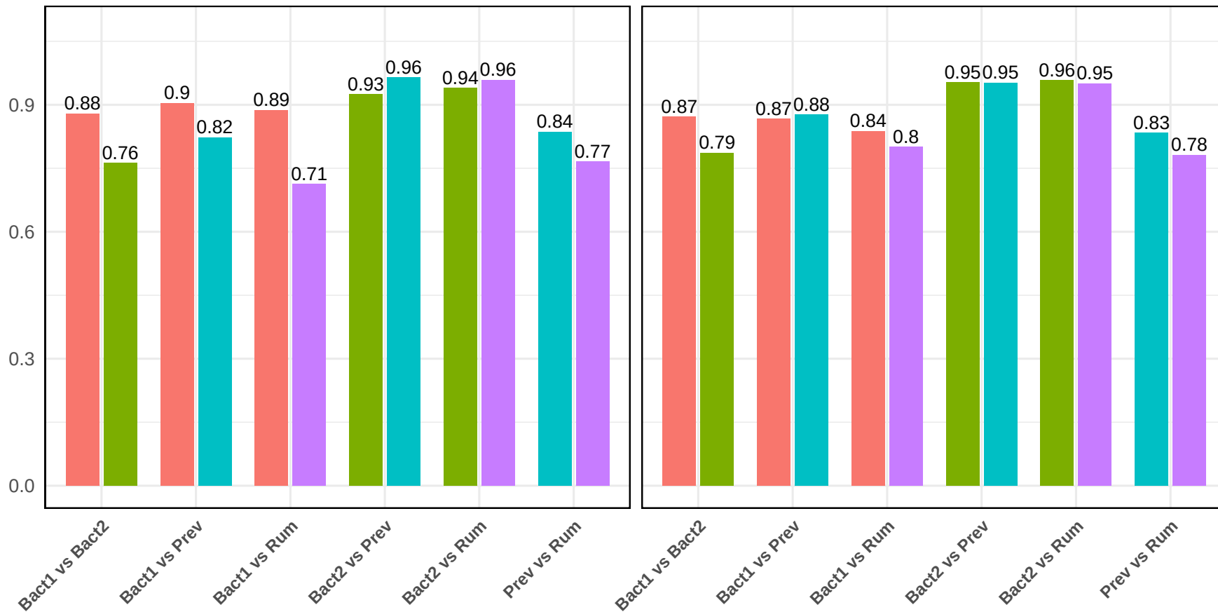
Recall
