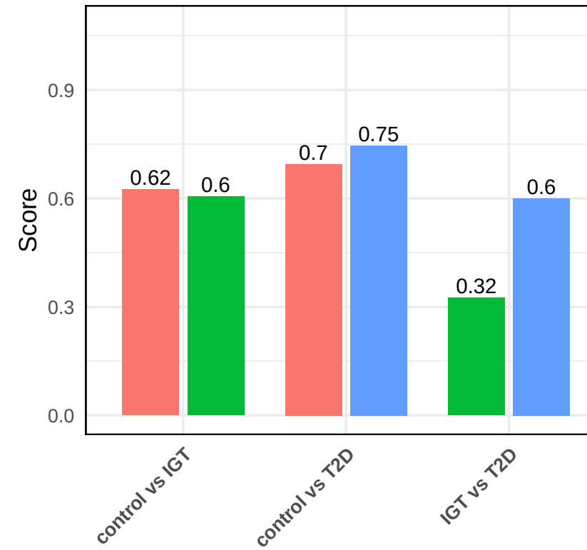
Recall
