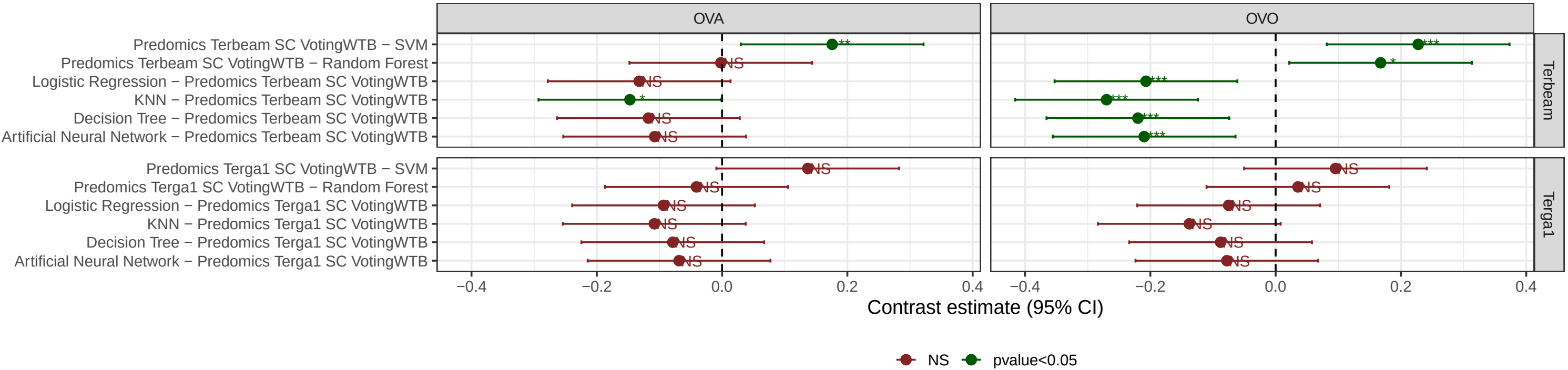
T2D – Contrasts (Test only): each SOTA method vs Predomics
