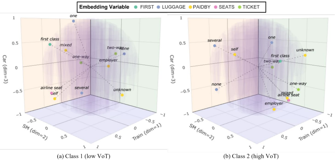
Figure 7 The focal model's class-specific embedding weight vectors for each category level, visualized on the unit sphere
