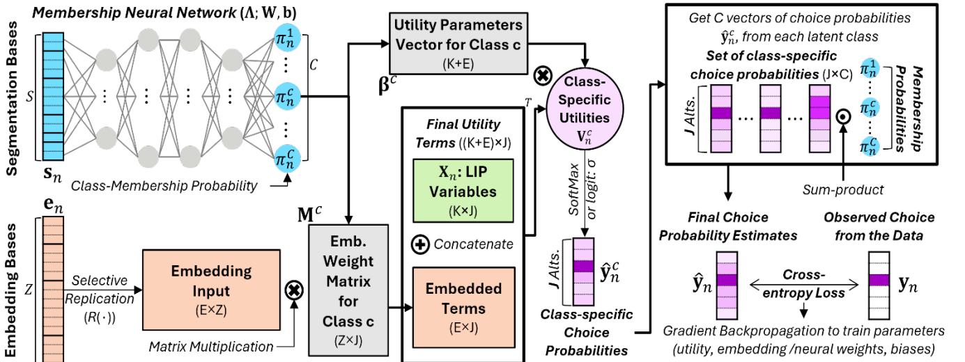
Figure 3 Overall computational flow of the DCM-SEAL architecture
