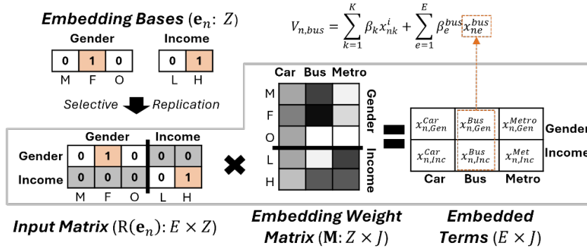
Figure 1 Example of embedding generation for categorical variables
