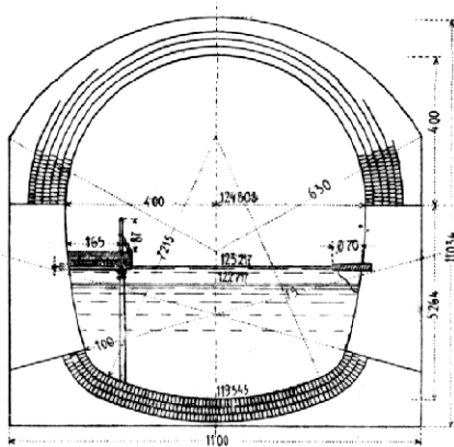
TUNNEL TORLONIUV
