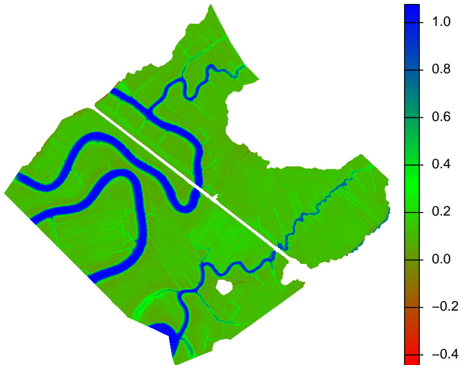
Proportion_Time_Inundated
