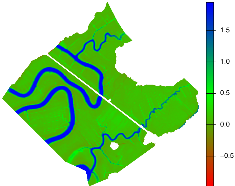
Percentile_95_Depth
