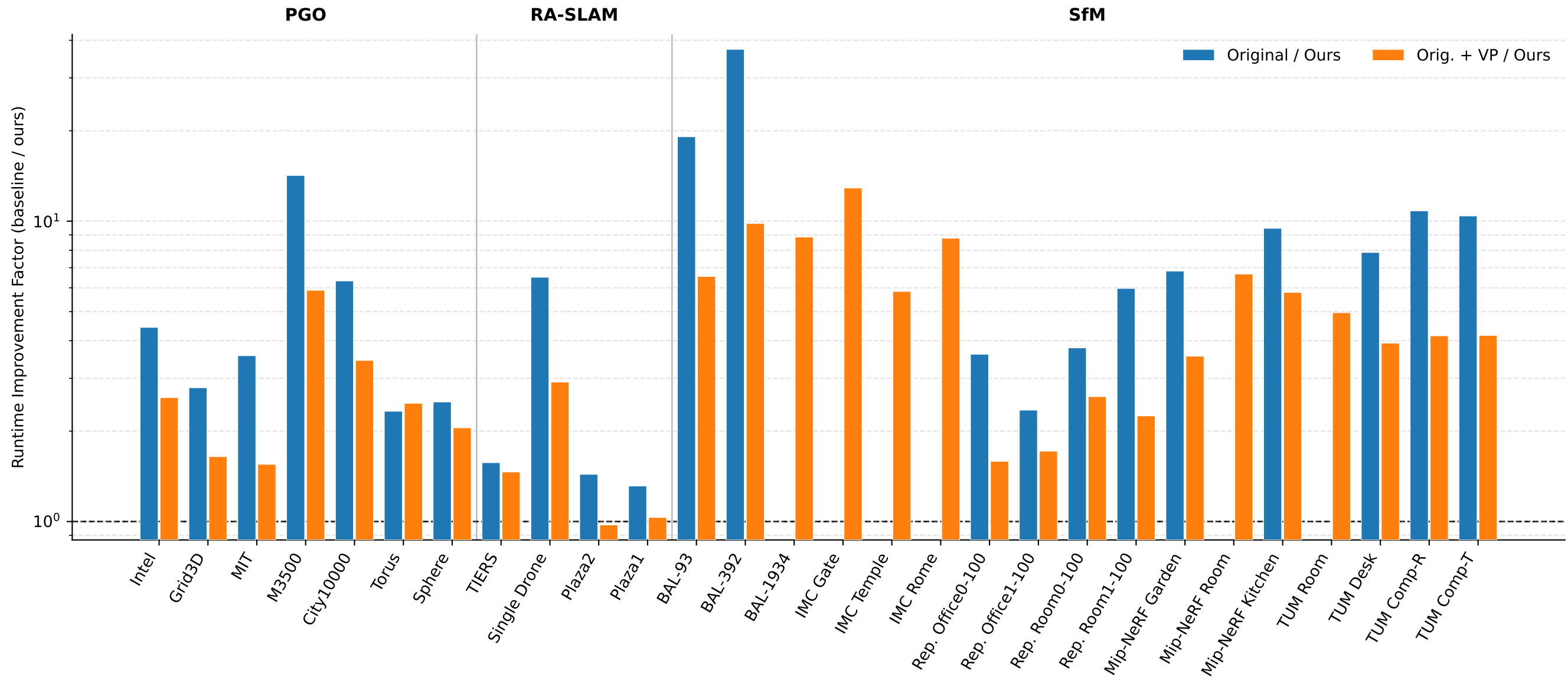
GPU Speedups Relative to Ours
