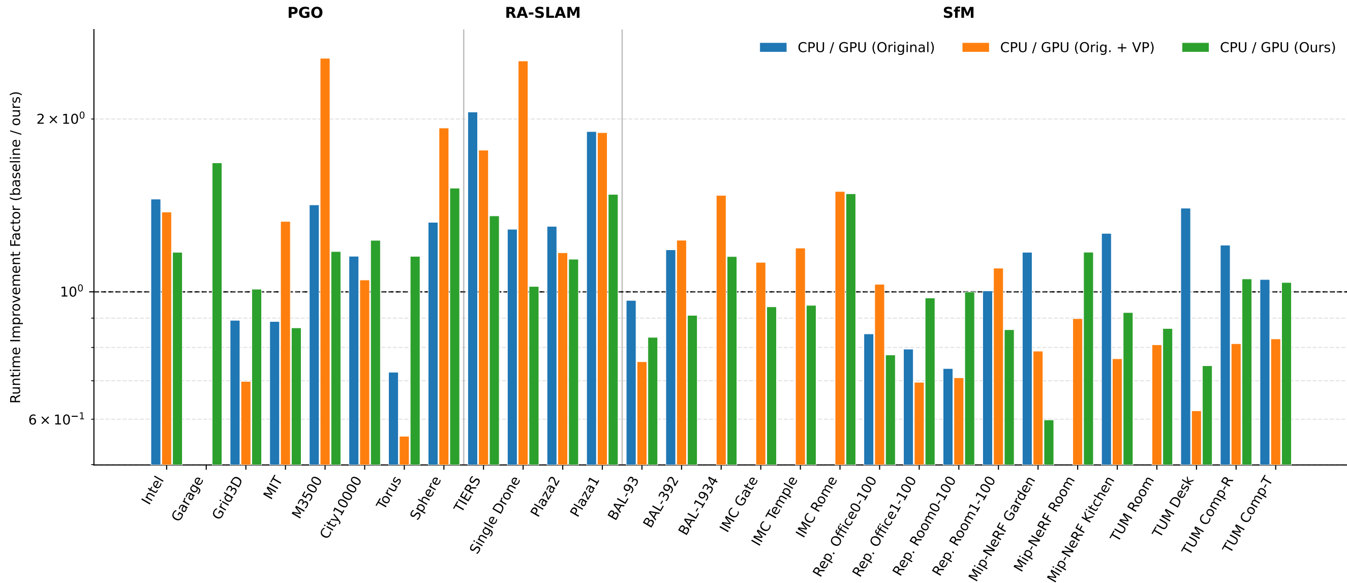
CPU-to-GPU Speedup by Method
