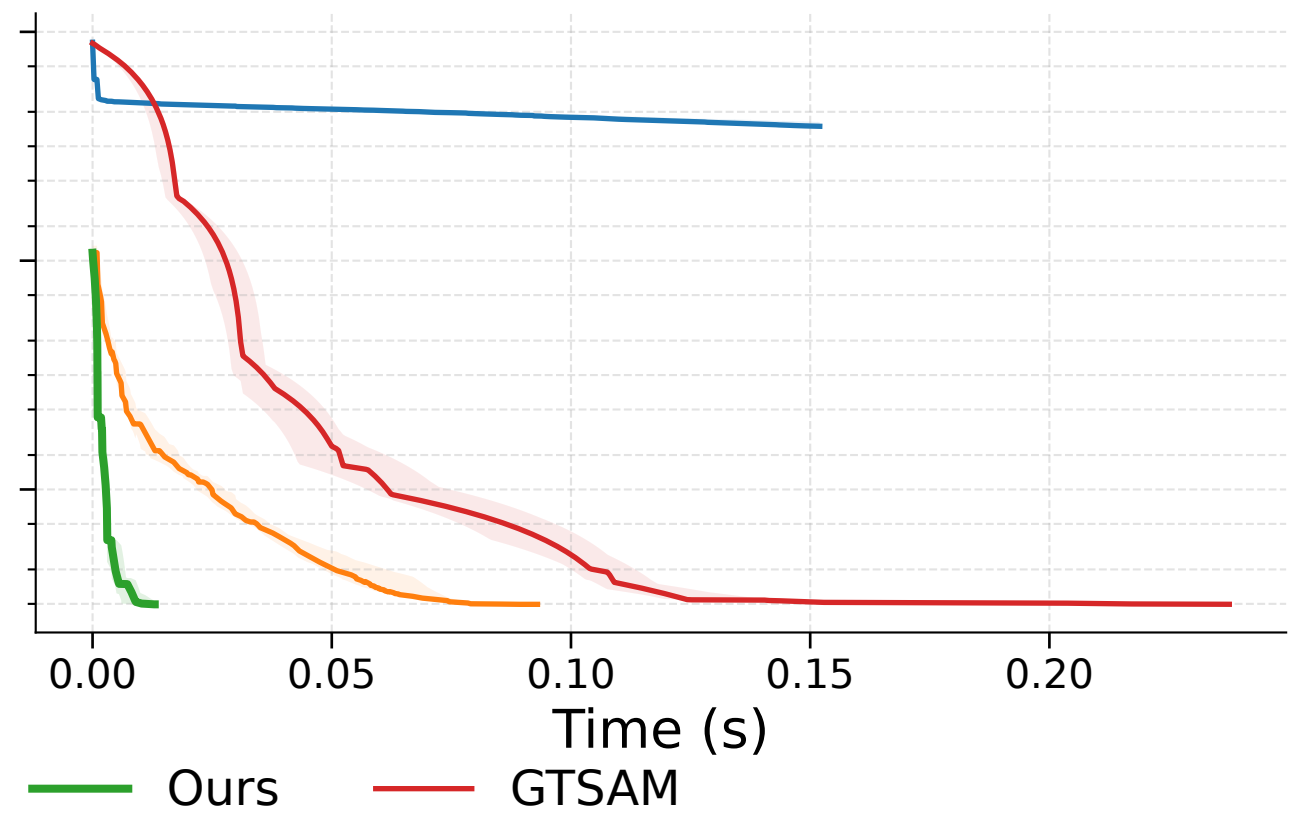
Solver Costs vs Time
