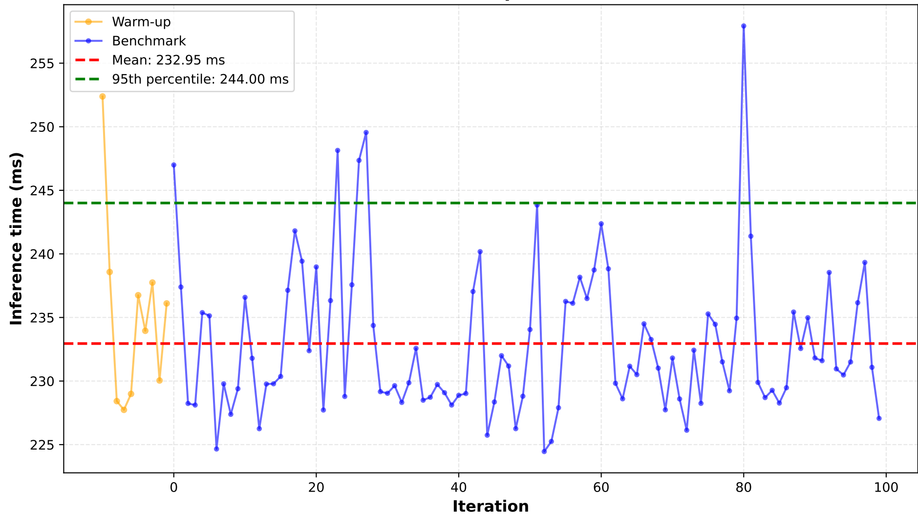
Inference time per iteration
