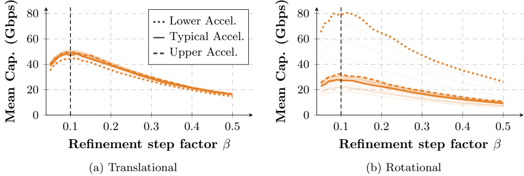
Figure 2: IMU-Assist parameter sensitivity to the refinement step factor \beta ( d_{\text{link}} = 3 m, Ideal Mechanical). Bold lines mark the Lower, Typical, and Upper Acceleration values: 0.5, 9.5, and 20 m/s 2 (translational); 0.5, 300, and 700 deg/s 2 (rotational).
