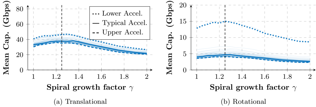
Figure 1: Hierarchical Search parameter sensitivity to the spiral growth factor \gamma ( d_{\text{link}} = 3 m, Ideal Mechanical). Bold lines mark the Lower, Typical, and Upper Acceleration values: 0.5, 9.5, and 20 m/s 2 (translational); 0.5, 300, and 700 deg/s 2 (rotational).
