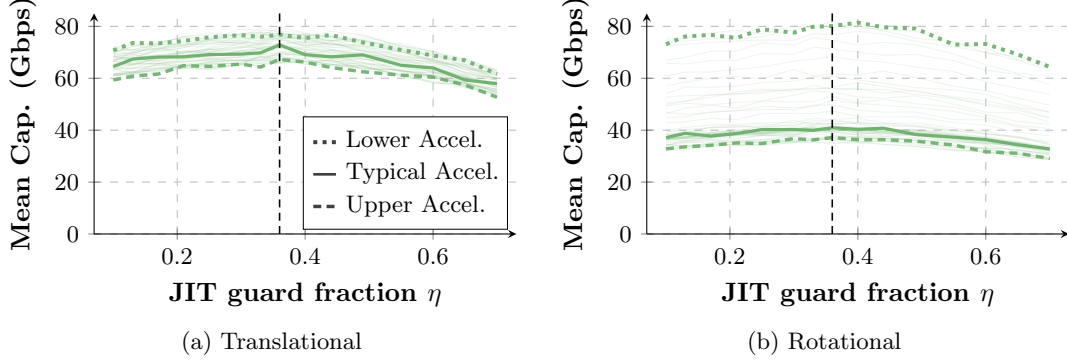
Figure 3: JIT guard fraction \eta sensitivity ( d_{\text{link}} = 3 m, Ideal Mechanical). Bold lines mark the Lower, Typical, and Upper Acceleration values: 0.5, 9.5, and 20 \text{m/s}^2 (translational); 0.5, 300, and 700 \text{deg/s}^2 (rotational).
