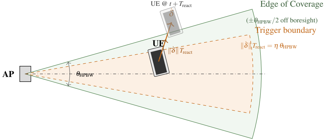
Figure 11. Edge of Coverage (EoC, at \pm \theta_{\text{HPBW}}/2 off boresight) and JIT's trigger boundary, defined implicitly by \|\dot{\delta}\| T_{\text{react}} = \eta \theta_{\text{HPBW}} . The UE evaluates the trigger condition locally at every IMU sample. Faster motion contracts the boundary toward boresight; slower motion expands it toward the EoC.
