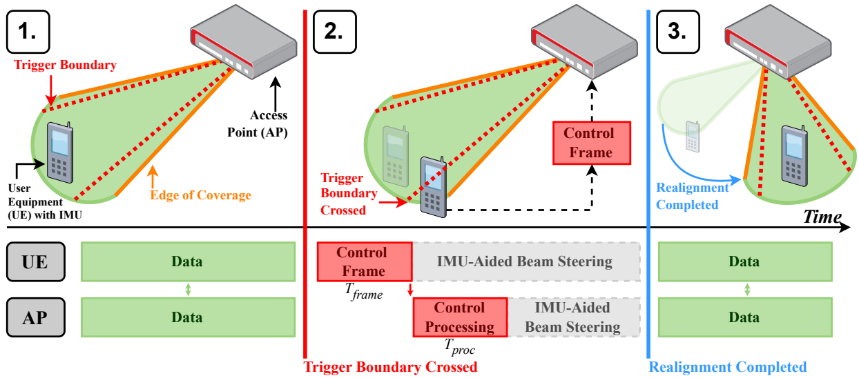
Figure 1. Overview of JIT proactive beam management. (1) Steady-state operation with continuous RF and IMU monitoring. (2) Upon crossing the trigger boundary, the UE transmits a control frame ( T_{frame} ) containing its kinematic state just before exiting the Edge of Coverage; the AP processes it ( T_{proc} ) and both nodes initiate beam steering. (3) Realignment completes and the data link is restored. The bottom timeline shows the UE and AP activity during the procedure.
