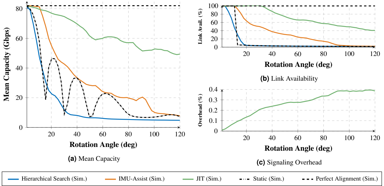
Figure 7. Effect of total angular displacement ( 1^\circ – 120^\circ ) at fixed rotational acceleration ( 120 \text{ deg/s}^2 ), Ideal Mechanical. (c) Overhead plateaus at \sim 0.39\% above 90^\circ as realignment frequency saturates.
