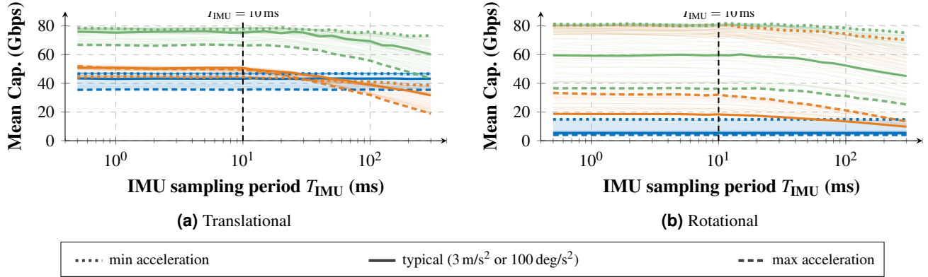
Figure 14. Mean capacity vs. IMU sampling period T_{\text{IMU}} , Ideal Mechanical steering ( d_{\text{link}} = 3 m). Bold lines mark the min, typical, and max accelerations; vertical dashed lines mark the Table 2 baseline T_{\text{IMU}} = 10 ms.
