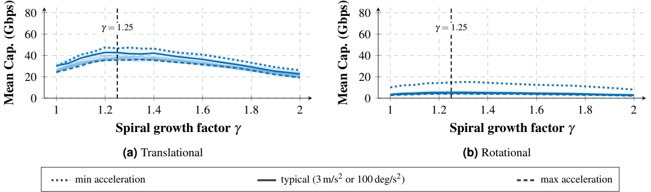
Figure 10. Hierarchical Search parameter sensitivity to the spiral growth factor \gamma ( d_{\text{link}} = 3 \text{ m} , Ideal Mechanical). Bold lines mark the min, typical, and max accelerations.
