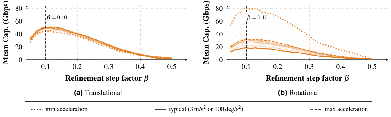
Figure 12. IMU-Assist parameter sensitivity to the refinement step factor \beta ( d_{\text{link}} = 3 m, Ideal Mechanical). Bold lines mark the min, typical, and max accelerations.
