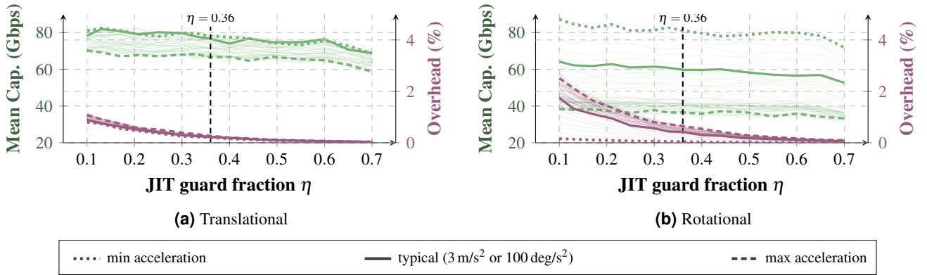
Figure 13. JIT guard fraction \eta sensitivity ( d_{\text{link}} = 3\text{ m} , Ideal Mechanical). Bold lines mark the min, typical, and max accelerations.
