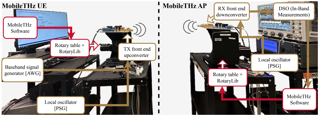
Figure 15. MobileTHz HIL testbed. The UE (left) and AP (right) each pair a sub-THz RF front-end with a dual-axis rotary stage. A 9-axis IMU on the UE supplies inertial data for the IMU-Assisted and JIT algorithms.
