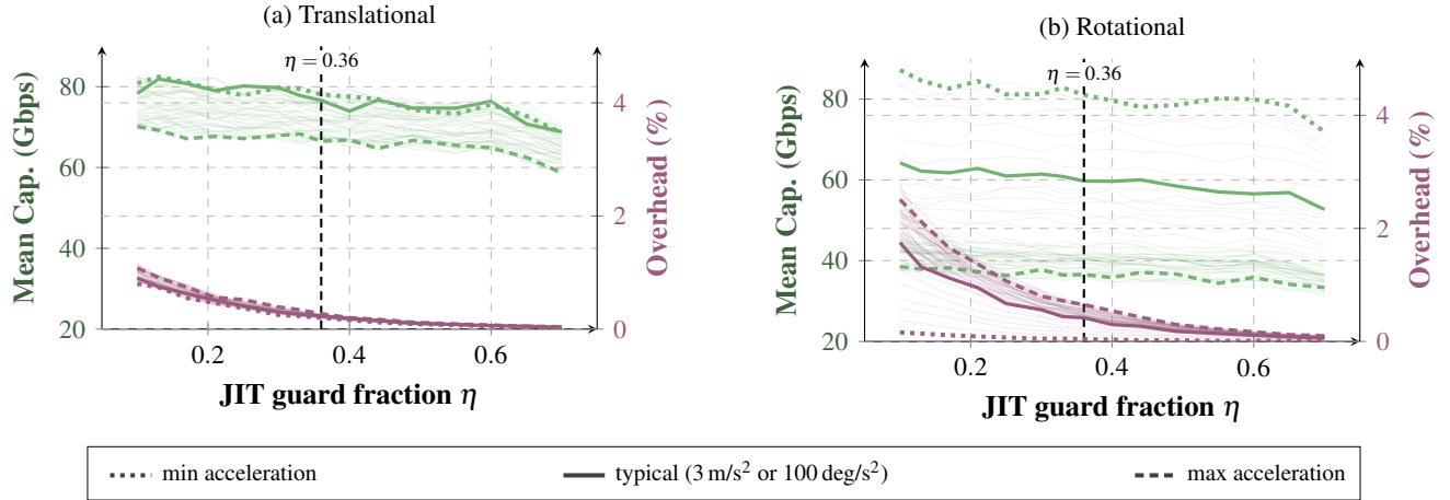
Figure 13. JIT guard fraction \eta sensitivity, Ideal Mechanical steering. (a) Translational; (b) Rotational. Each panel overlays mean capacity (left axis) and signaling overhead (right axis). Mean capacity stays within \pm 5\% of the maximum across the plateau \eta \in [0.20, 0.50] at every acceleration shown.
