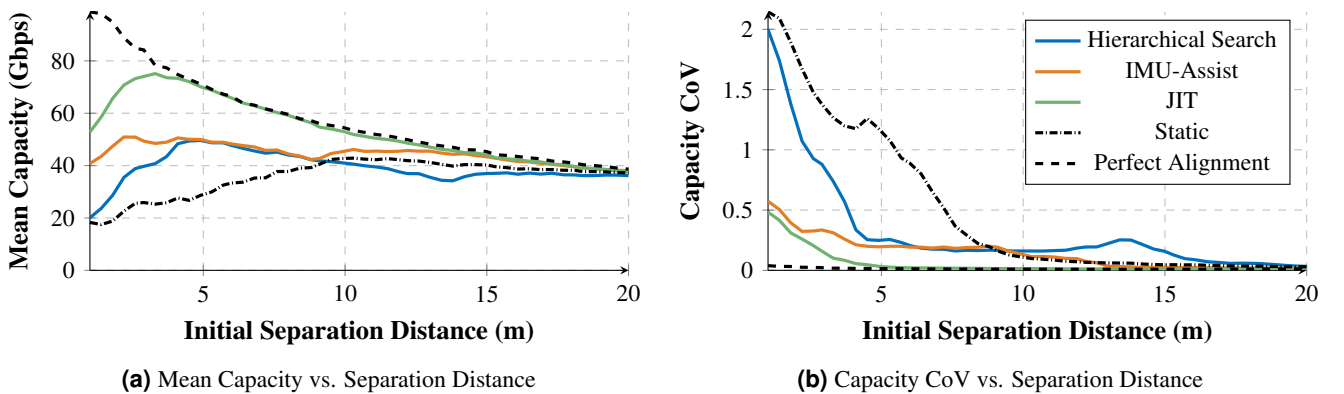
Figure 6. Effect of initial AP–UE separation (1–20 m) on a fixed translational pass-by ( D_{\text{traversed}} = 1.5 m, 3.0 \text{m/s}^2 peak), Ideal Mechanical. Performance converges beyond \sim 10 m as path loss, not alignment, becomes the limiting factor.
