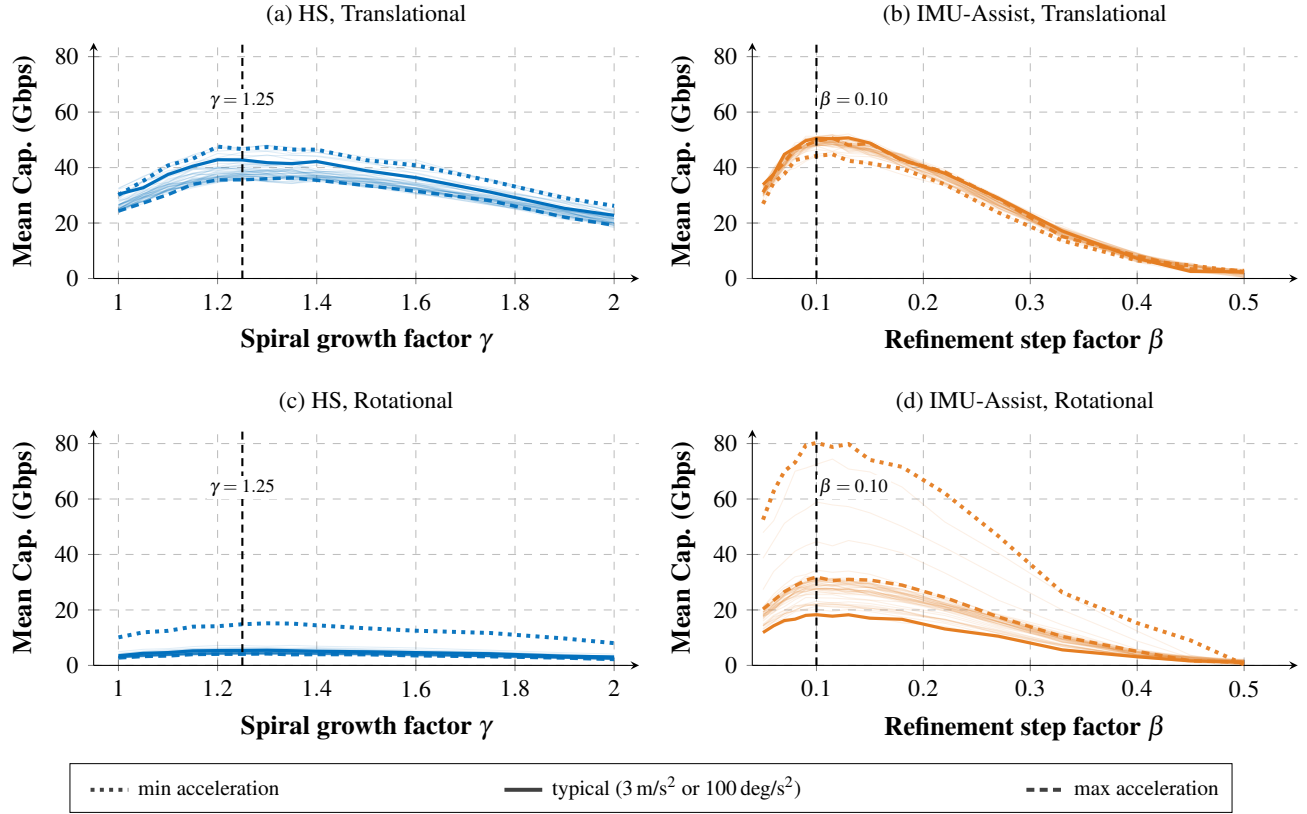
Figure 12. Baseline parameter sensitivity, Ideal Mechanical steering. Rows: translational (top), rotational (bottom). Columns: (a,c) Hierarchical Search vs. \gamma ; (b,d) IMU-Assist vs. \beta . Bold lines mark the min, typical, and max accelerations. The chosen \gamma = 1.25 and \beta = 0.10 lie within \pm 10\% of the peak at every acceleration shown.
