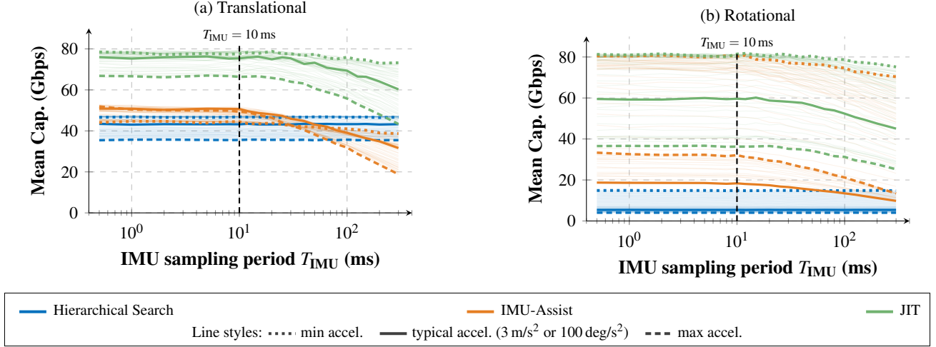
Figure 14. Mean capacity vs. IMU sampling period T_{\text{IMU}} , Ideal Mechanical steering ( d_{\text{link}} = 3 m). (a) Translational; (b) Rotational. Bold lines mark the min, typical, and max accelerations; vertical dashed lines mark the Table 3 baseline T_{\text{IMU}} = 10 ms.
