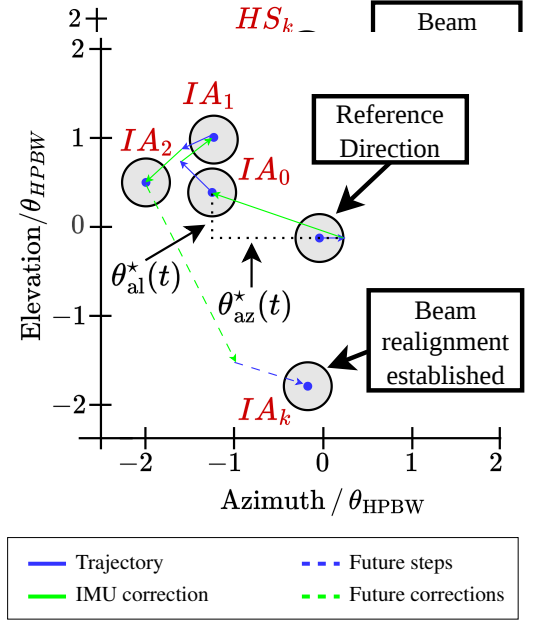
Figure 10. IMU-Assisted search trajectory. IMU corrections (green) shift the search center to the sensor-predicted LoS direction before each spiral step. The local refinement spiral (blue) scans around the corrected center.
