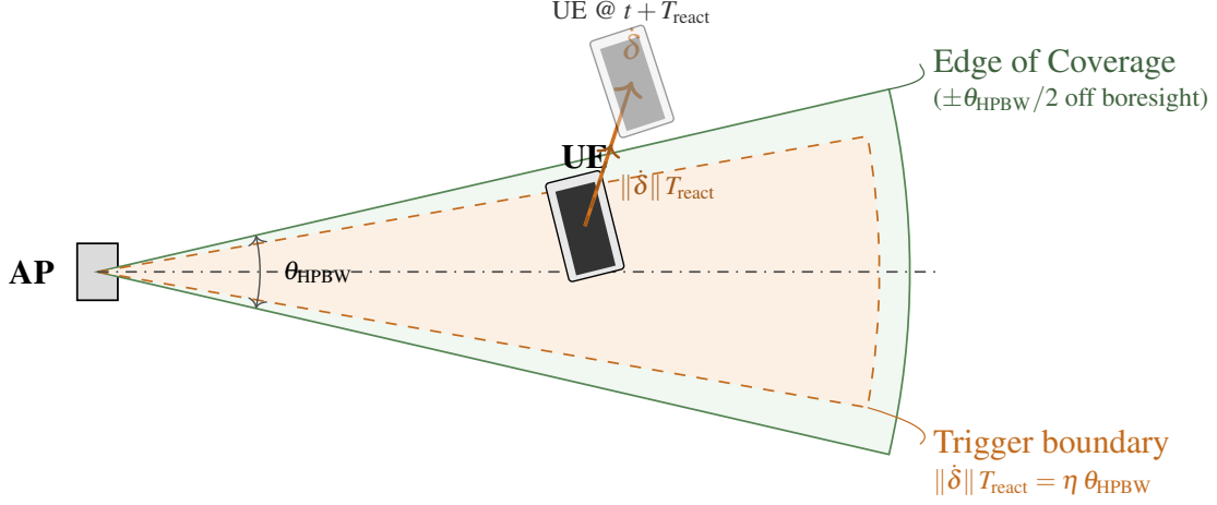
Figure 11. Edge of Coverage (EoC, at \pm\theta_{\text{HPBW}}/2 off boresight) and JIT’s trigger boundary, defined implicitly by \|\dot{\delta}\| T_{\text{react}} = \eta \theta_{\text{HPBW}} . The UE evaluates the trigger condition locally at every IMU sample. Faster motion contracts the boundary toward boresight; slower motion expands it toward the EoC.
