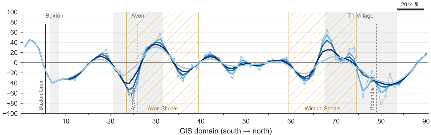
Total shoreline change, 1996–2015 (CoastSat LRR 1996–2015 \times 19 yr, every LOWESS width)
