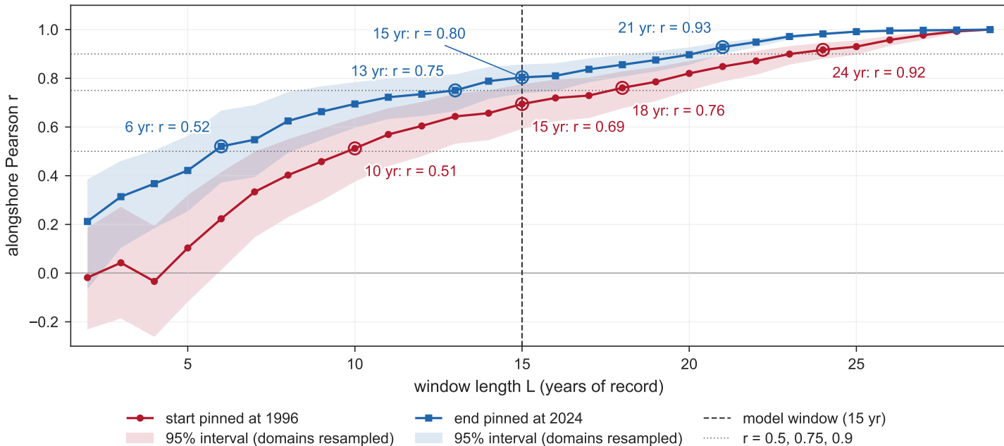
Alongshore correlation of windowed shoreline change rates with the 1996–2024 rate
