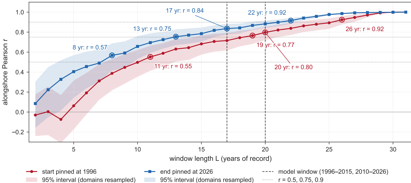
Alongshore correlation of windowed shoreline change rates with the 1996–2026 rate
