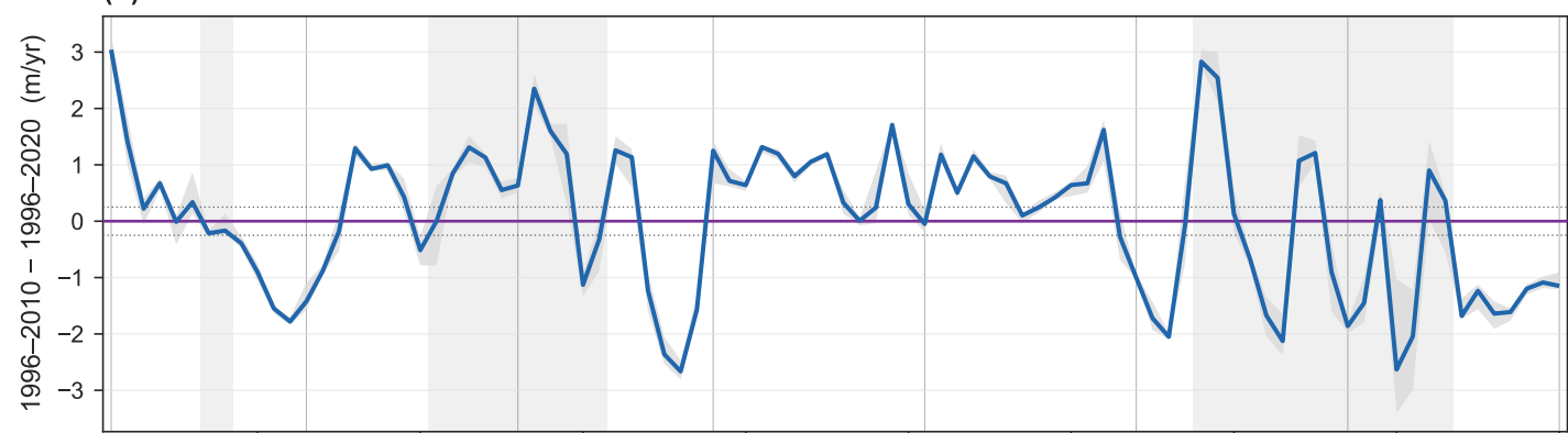
Transects whose 1996–2010 rate is already in the band
