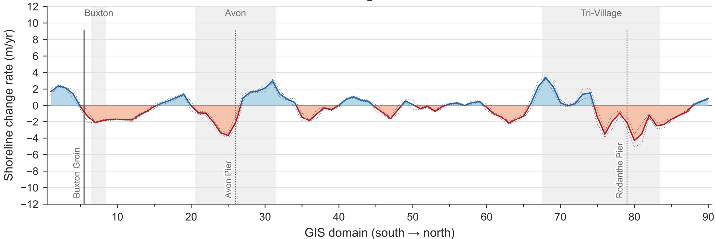
Shoreline change rate, 1996–2015
