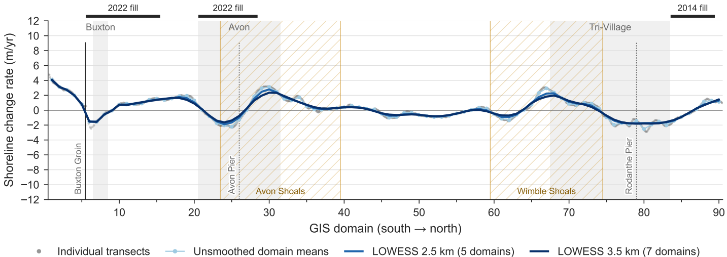
Shoreline change rate, 1996–2026: LOWESS smoothing at 2.5 km and 3.5 km
