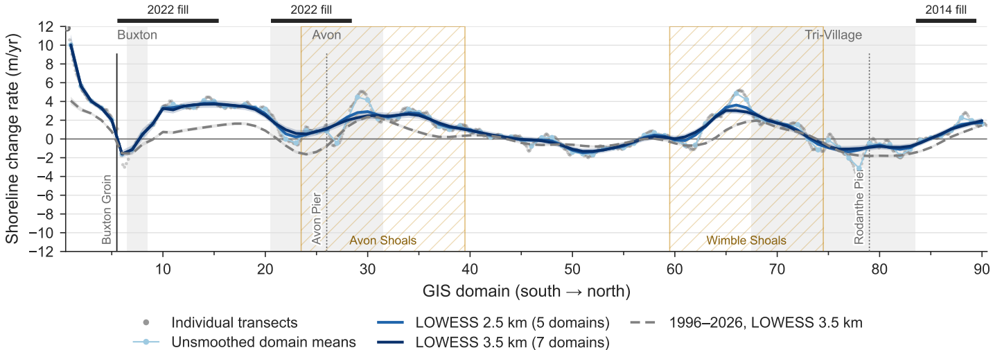
Shoreline change rate, 2010–2026: LOWESS smoothing at 2.5 km and 3.5 km
