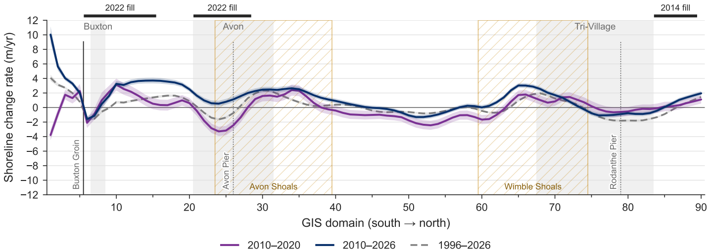
Shoreline change rate, 2010–2020 and 2010–2026, against the 1996–2026 rate (LOWESS 3.5 km)
