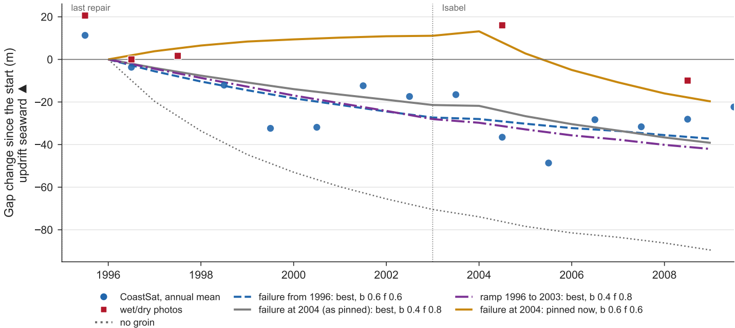
Calibration 1996-2009: gap across the groin
