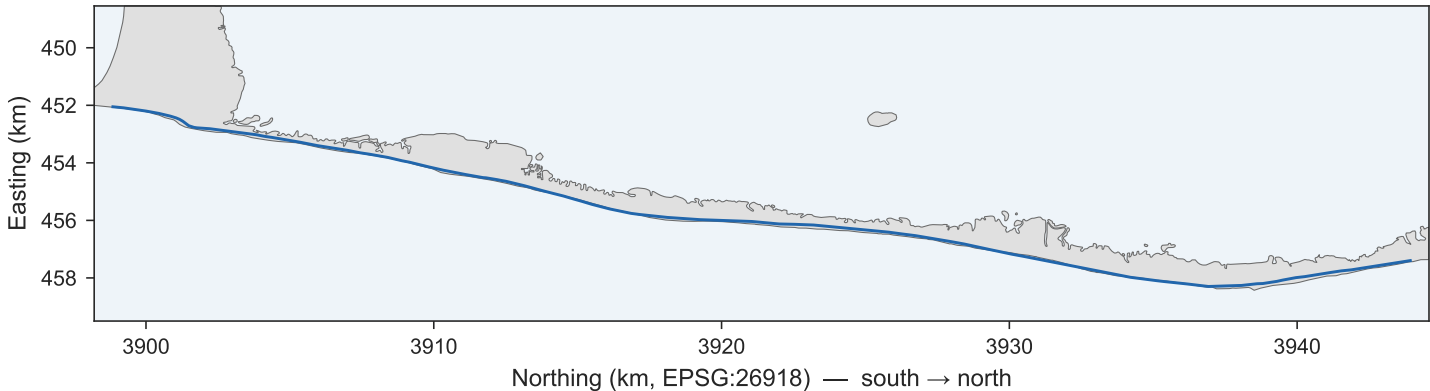
Mean shoreline, 1995-10-12 – 1997-10-12
