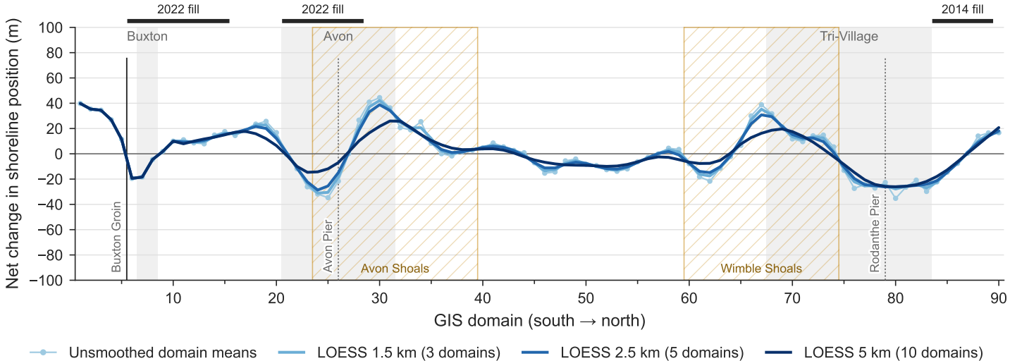
Projected shoreline change, 2010–2024 (CoastSat LRR 1996–2024 \times 14 yr, every LOESS width)
