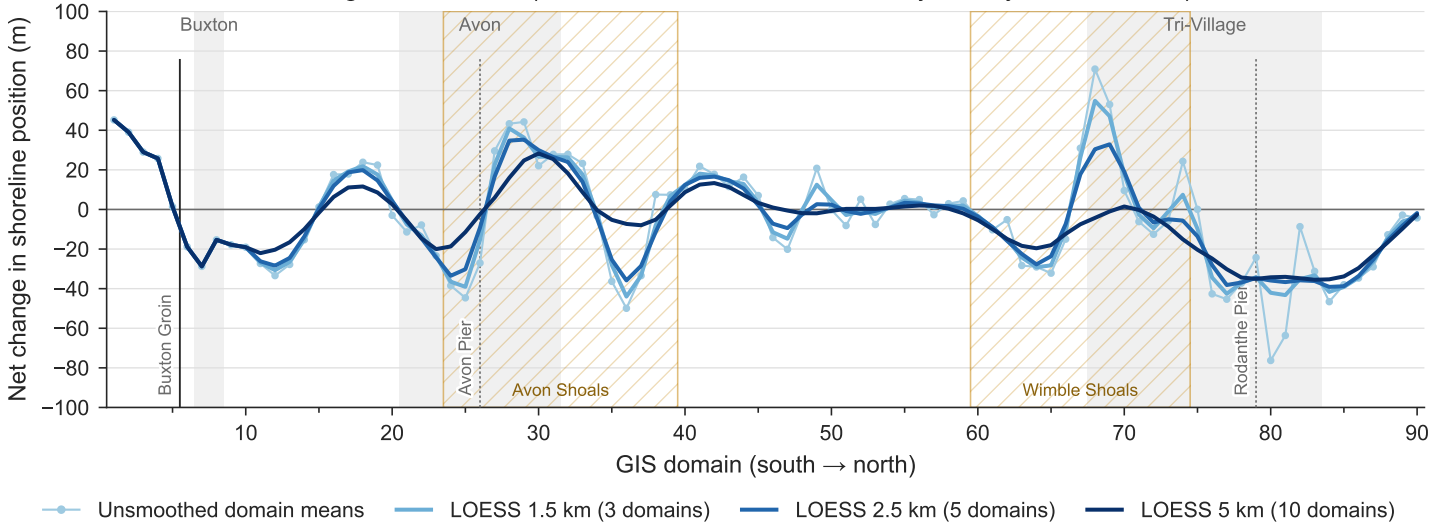
Total shoreline change, 1996–2010 (CoastSat LRR 1996–2010 \times 14 yr, every LOESS width)
