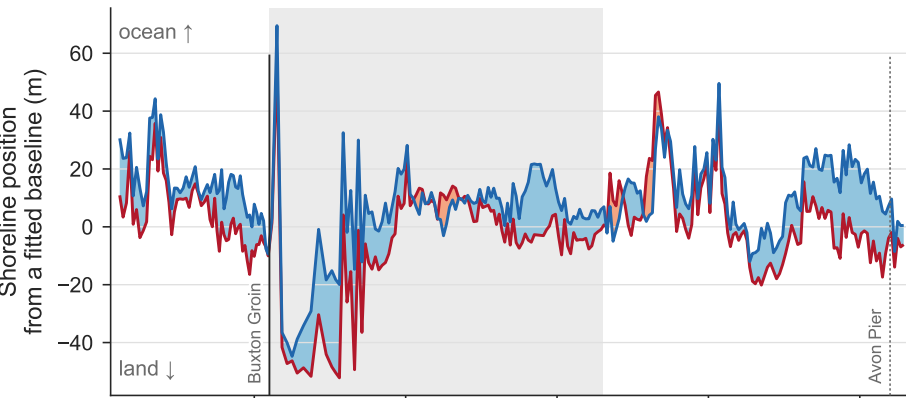
(a) Shorelines, the year before and the year after
