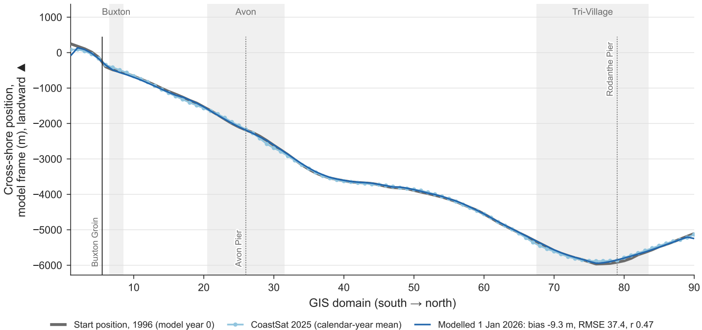
Full management, no groin, edgeBE: the 1996 start, CoastSat 2025 and the modelled end shoreline
