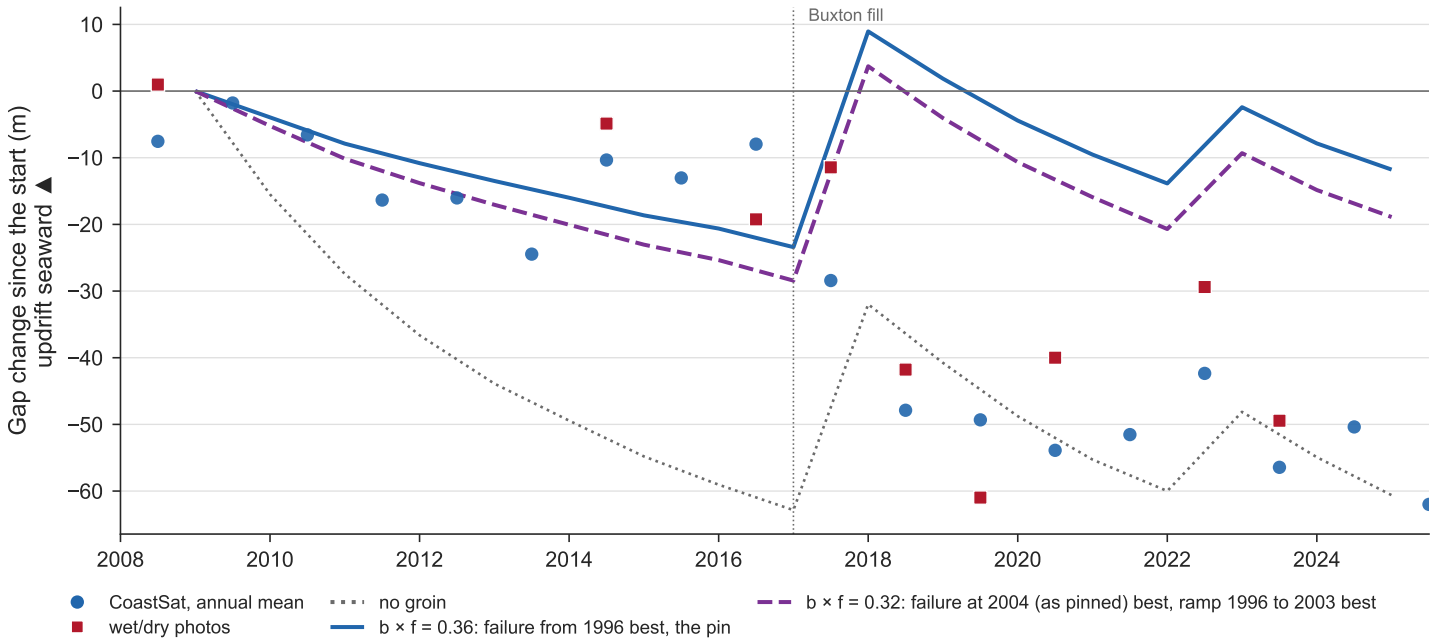
Test 2009-2025: gap across the groin (not fitted)
