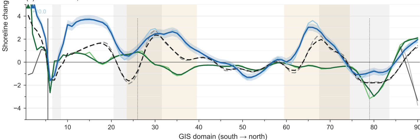
(b) Test window, 2010–2026
