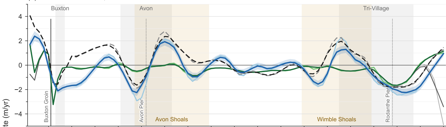
(b) Test window, 2010–2026
