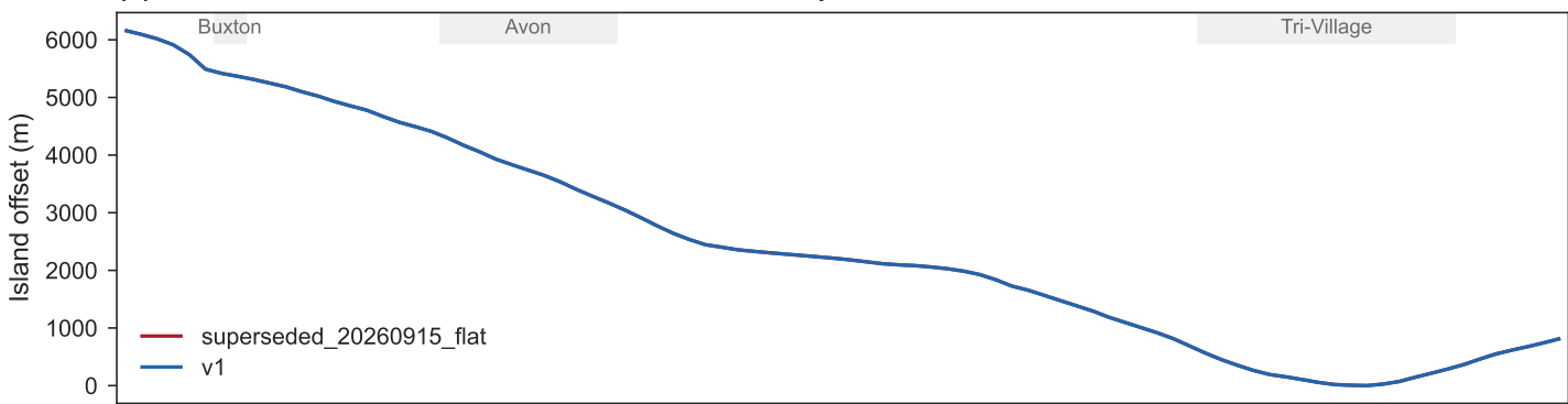
Island offset read by the model, 2004 start
