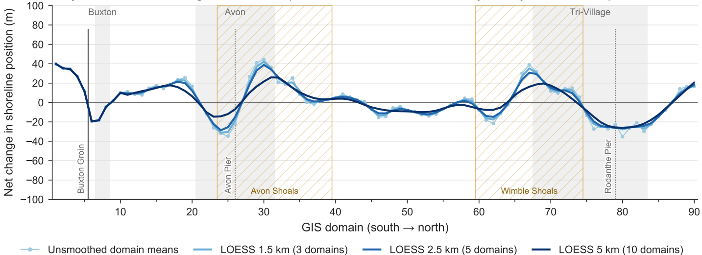
Projected shoreline change, 1996–2010 (CoastSat LRR 1996–2024 \times 14 yr, every LOESS width)
