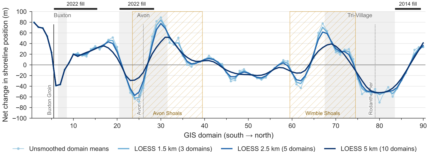
Total shoreline change, 1996–2024 (CoastSat LRR 1996–2024 \times 28 yr, every LOESS width)
