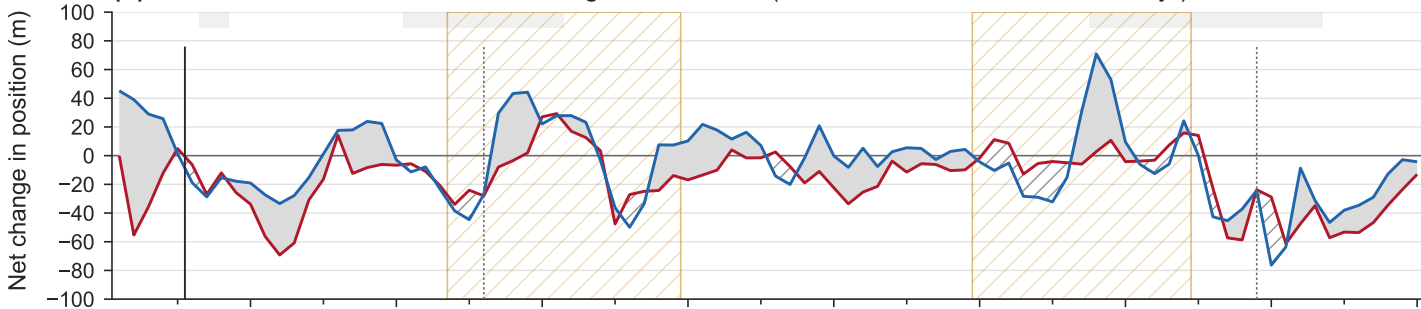
(c) Total shoreline change, 2010–2024 (CoastSat LRR 2010–2024 × 14 yr)
