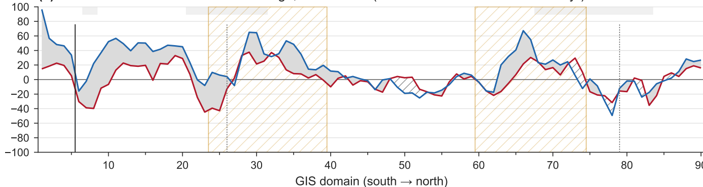
(c) Total shoreline change, 2010–2024 (CoastSat LRR 2010–2024 × 14 yr)
