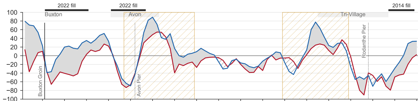
(b) Total shoreline change, 1996–2010 (CoastSat LRR 1996–2010 × 14 yr)
