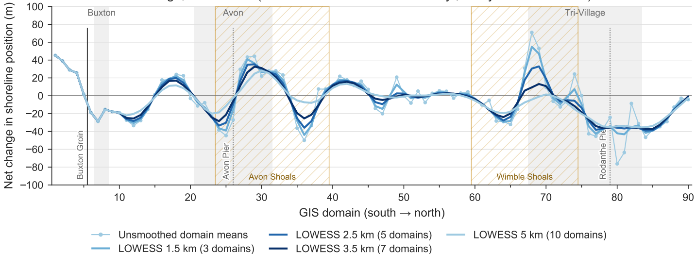
Total shoreline change, 1996–2010 (CoastSat LRR 1996–2010 \times 14 yr, every LOWESS width)
