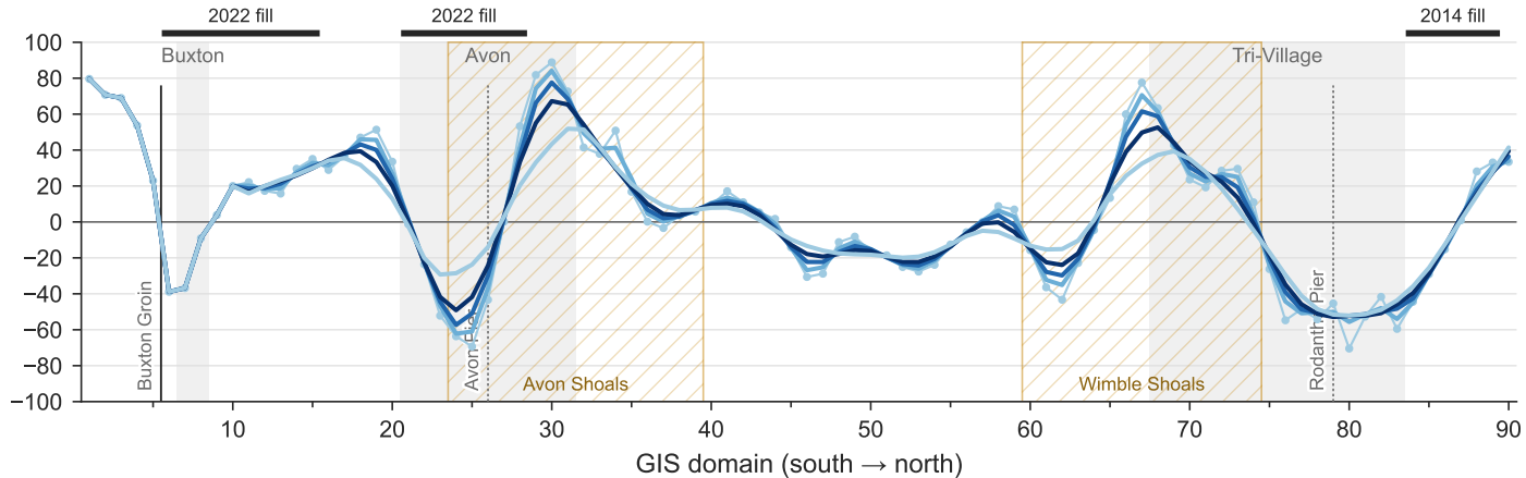
Total shoreline change, 1996–2024 (CoastSat LRR 1996–2024 \times 28 yr, every LOWESS width)
