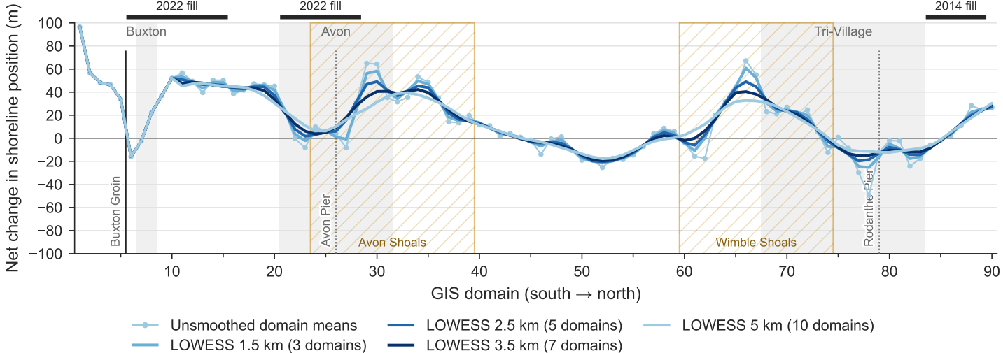
Total shoreline change, 2010–2024 (CoastSat LRR 2010–2024 \times 14 yr, every LOWESS width)
