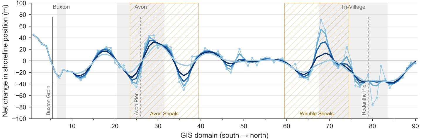
Total shoreline change, 1996–2010 (CoastSat LRR 1996–2010 \times 14 yr, every LOESS width)
