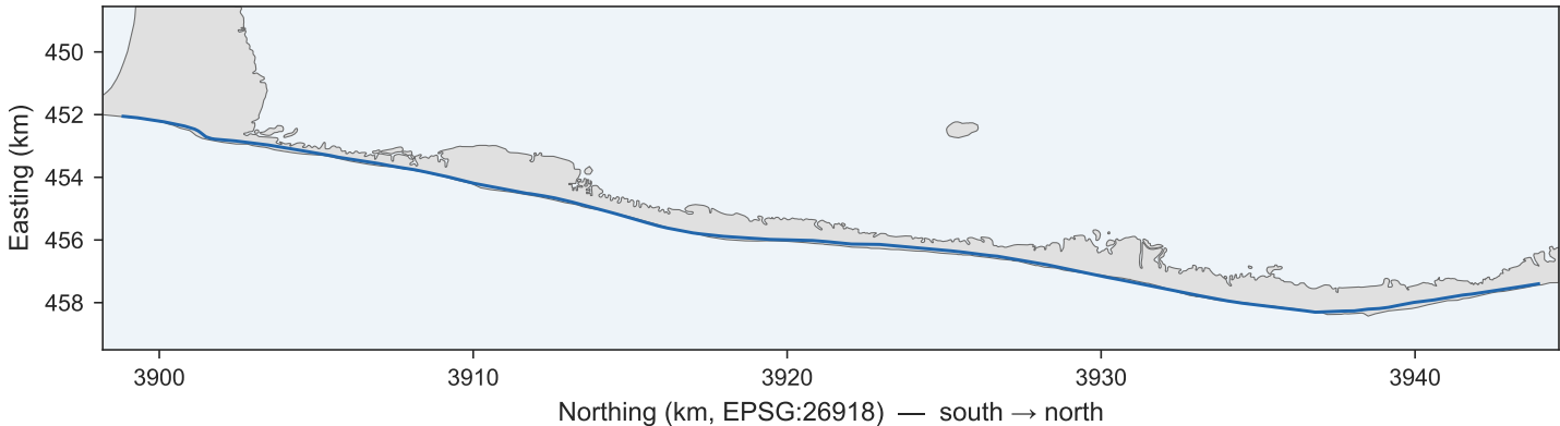
Mean shoreline, 1995–1997
