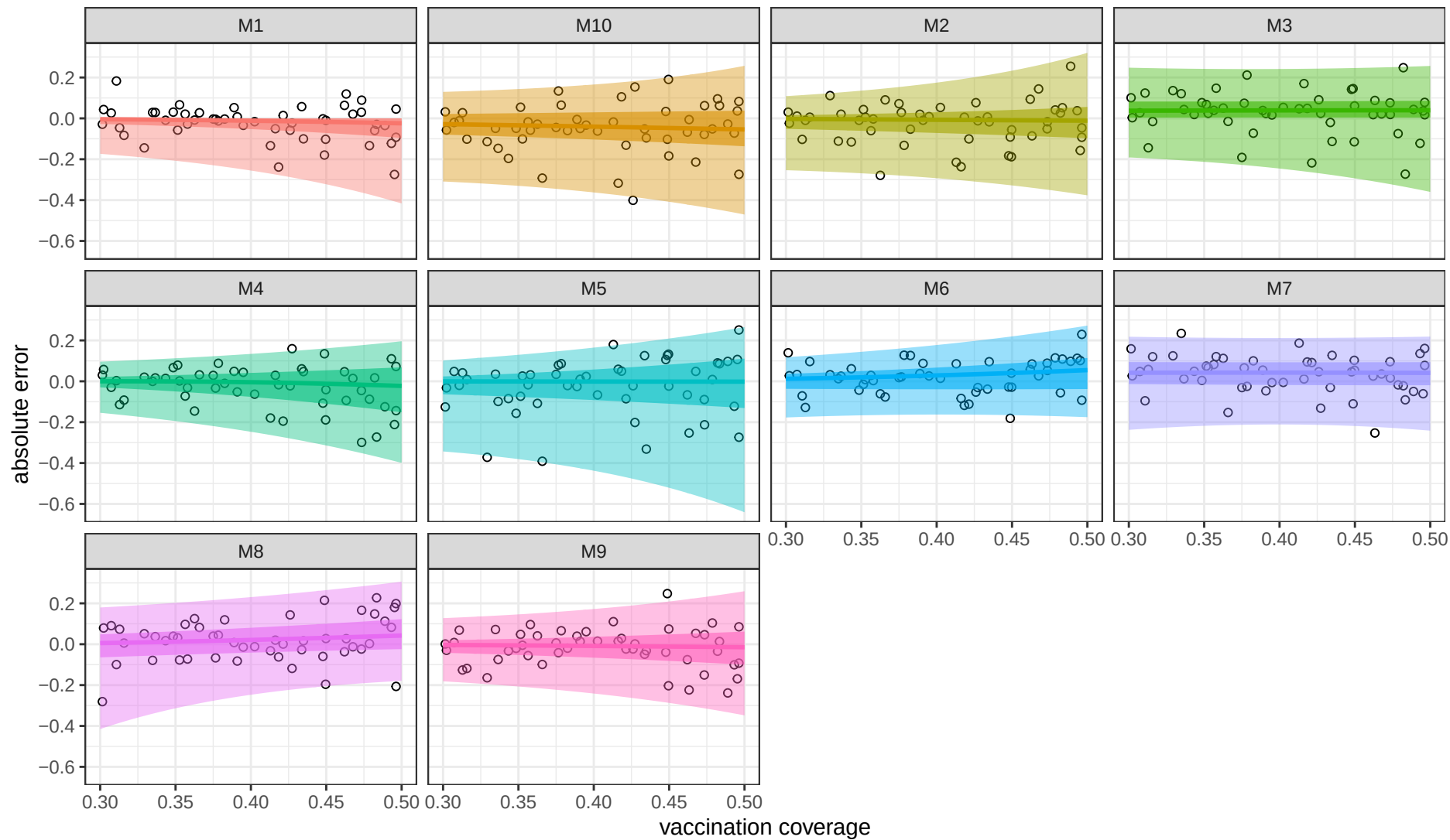
50 locations, high correlation between R0 and true vax (0.2)
