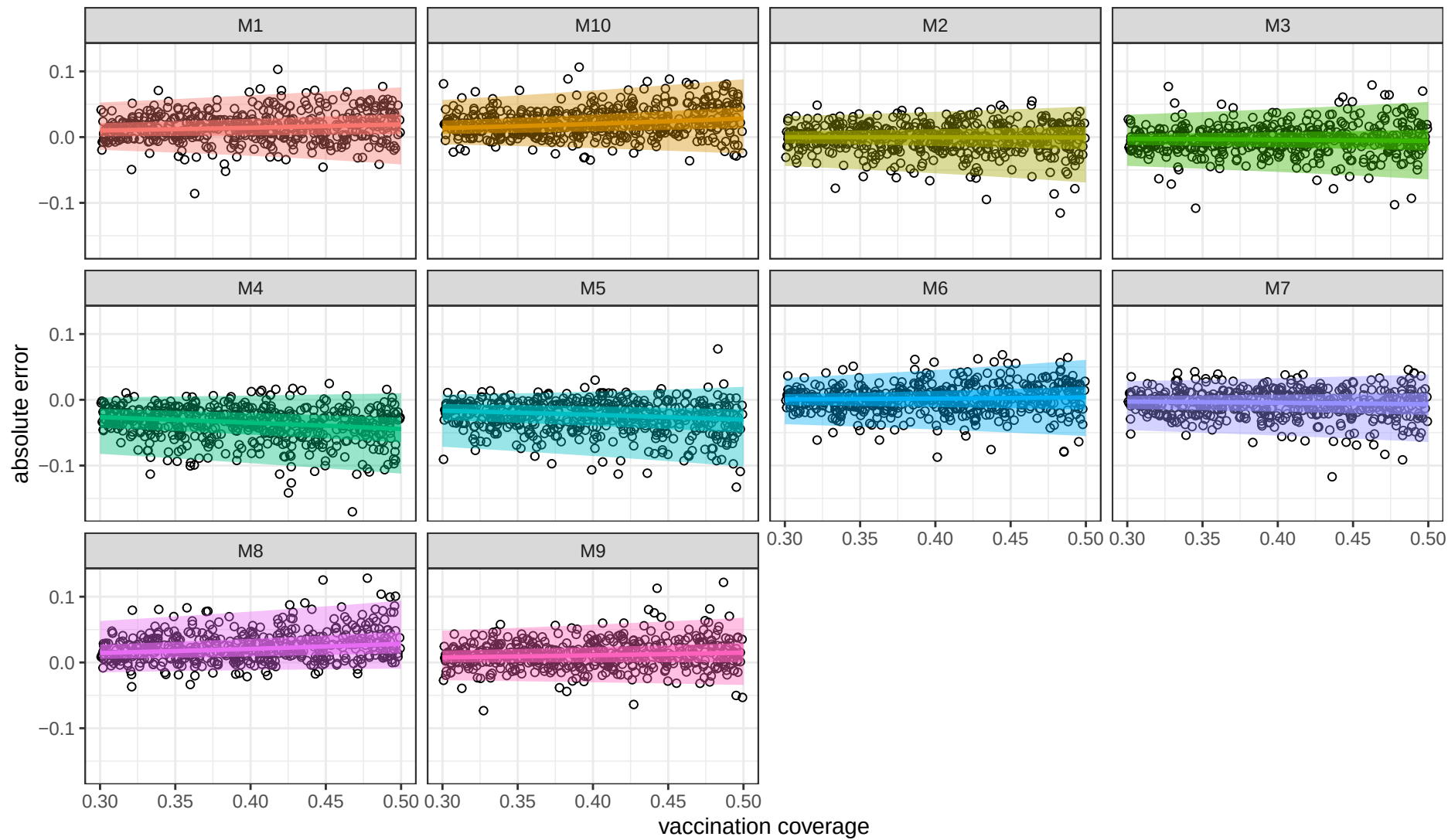
500 locations, low correlation between R0 and true vax (0.05)
