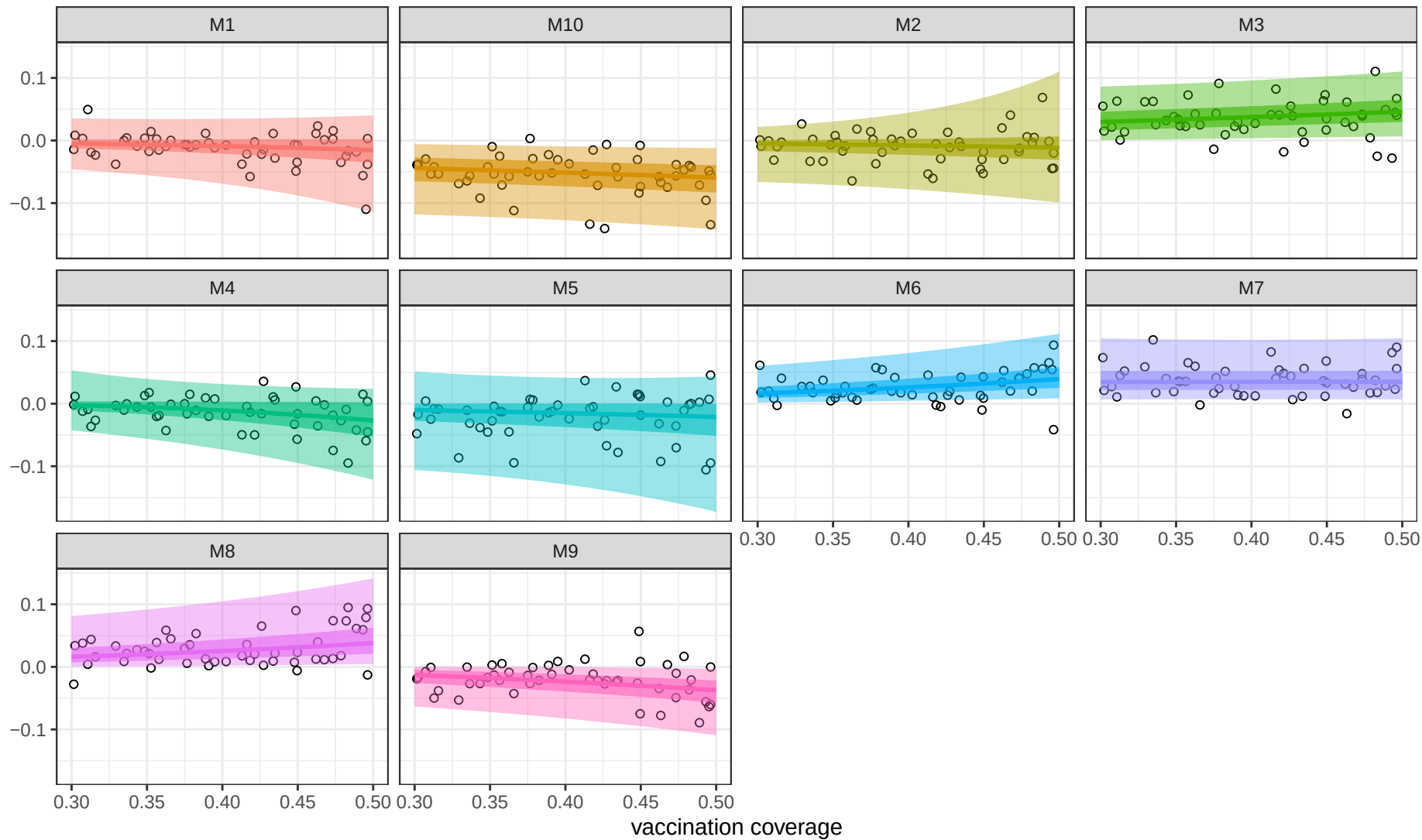
50 locations, low correlation between R0 and true vax (0.05)
