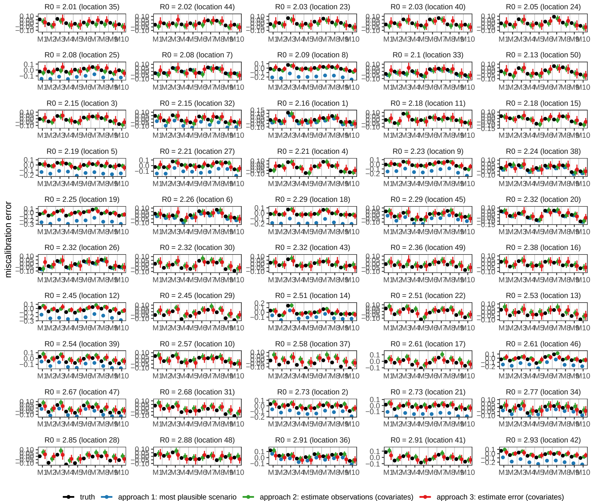
True and estimated miscalibration error in scenario 2
