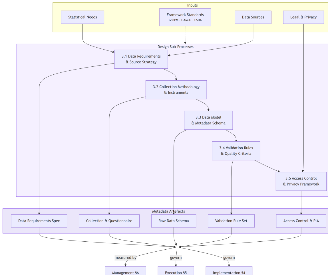
Figure 4: Design Process Decomposition. Statistical needs and framework standards flow into five design sub-processes, producing metadata artefacts that govern Implementation, Execution, and Management.
