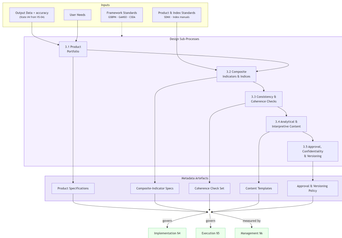
Figure 4: Design Process Decomposition. Output data with accuracy, user needs, and product standards flow into five design sub-processes, producing metadata artefacts that govern Implementation, Execution, and Management.
