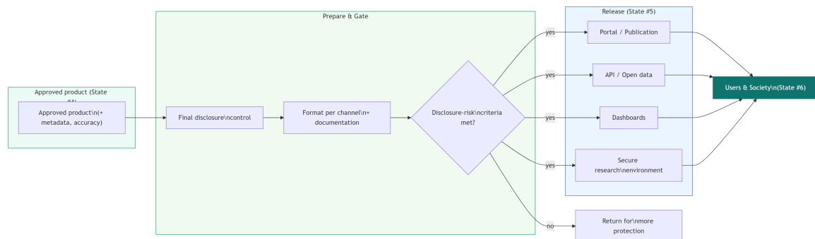
Figure 6: Release Architecture. The approved product is disclosure-controlled and formatted, must pass the disclosure-risk gate, and is then released through publication, API, dashboard, and secure research channels to users (State #6).
