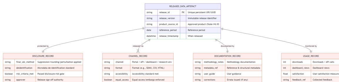
Figure 7: Released Data Artefact Structure. Each released version is linked to its disclosure-control record, the channels it was released via, its documentation, and its usage — all traceable to the approved product it came from.
