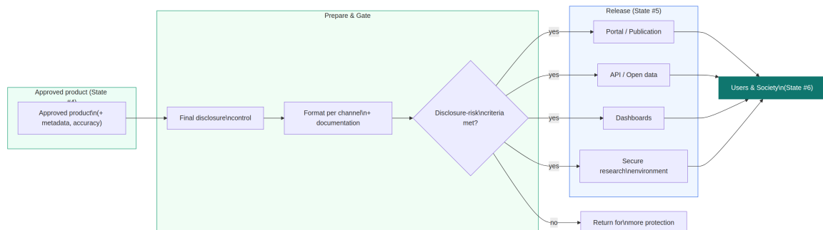
Figure 6: Release Architecture. The approved product is disclosure-controlled and formatted, must pass the disclosure-risk gate, and is then released through publication, API, dashboard, and secure research channels to users (State #6).
