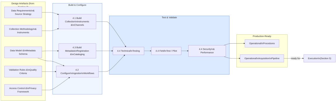
Figure 5: Implementation Pipeline from design artefacts through build/configure/test to production-ready system.
