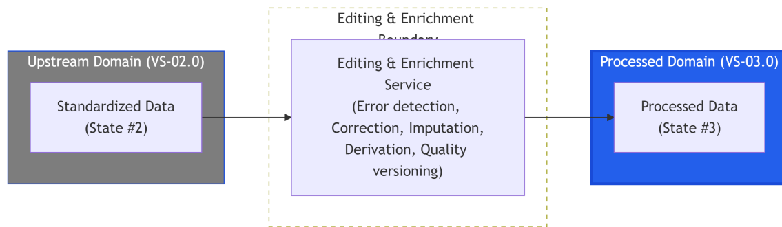
Figure 2: Steady State Transition from Standardized Data to Processed Data through the editing and enrichment service at the domain boundary.
