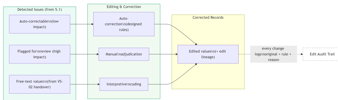
Figure 6: Editing and Correction Architecture. Auto-correctable, review-flagged, and free-text values are treated through automatic correction, manual adjudication, and interpretive coding respectively; every change writes original value, rule, and reason to the edit audit trail.
