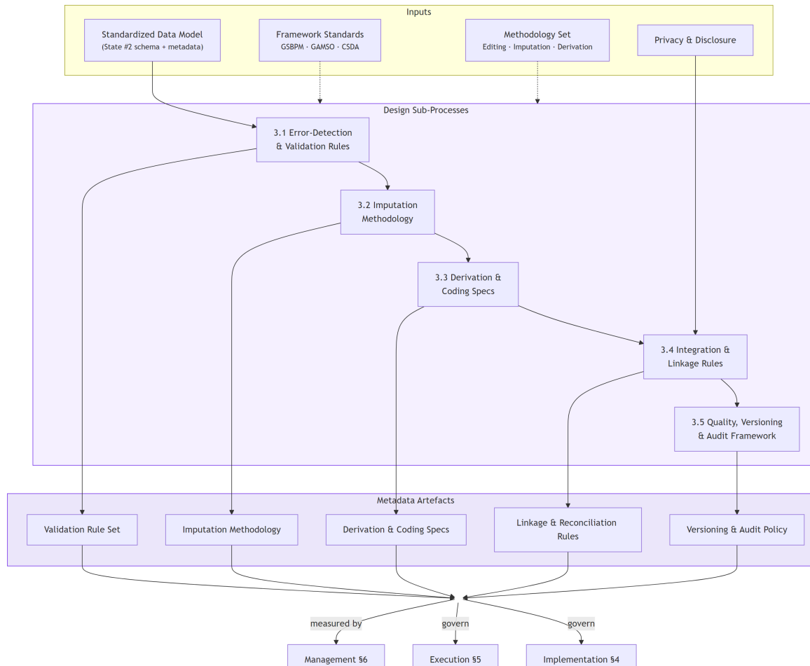
Figure 4: Design Process Decomposition. The standardized data model, methodology set, and framework standards flow into five design sub-processes, producing metadata artefacts that govern Implementation, Execution, and Management.
