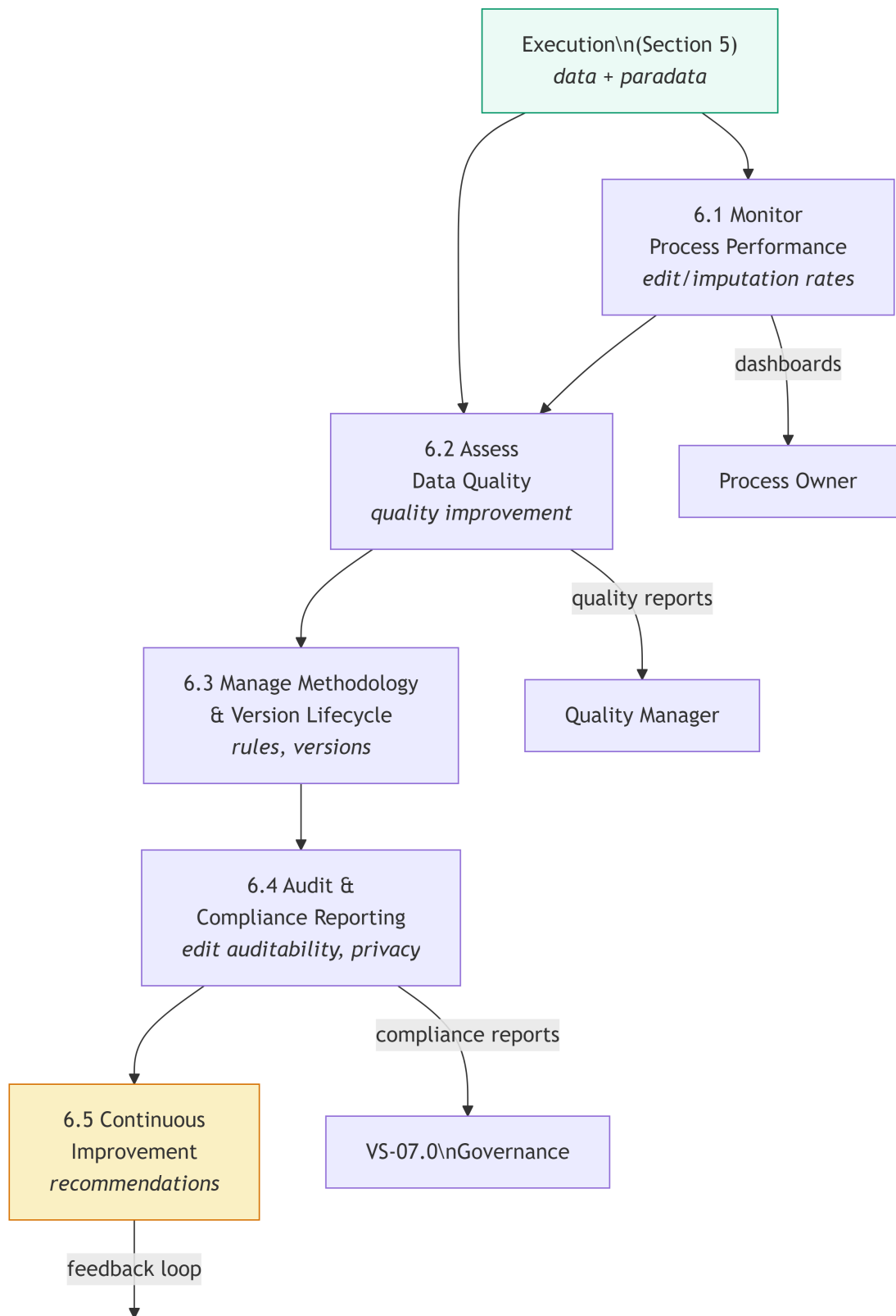
Figure 8: Management Feedback Loop. Execution data flows through monitoring, quality assessment, methodology/version management, and audit processes. Continuous improvement feeds recommendations back to Design, closing the governance cycle.
