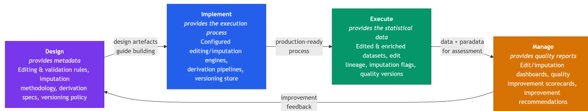
Figure 3: The Four-Process Governance Pattern. Each process type produces a distinct artefact class. The cycle closes when Management findings feed back into Design improvements.
