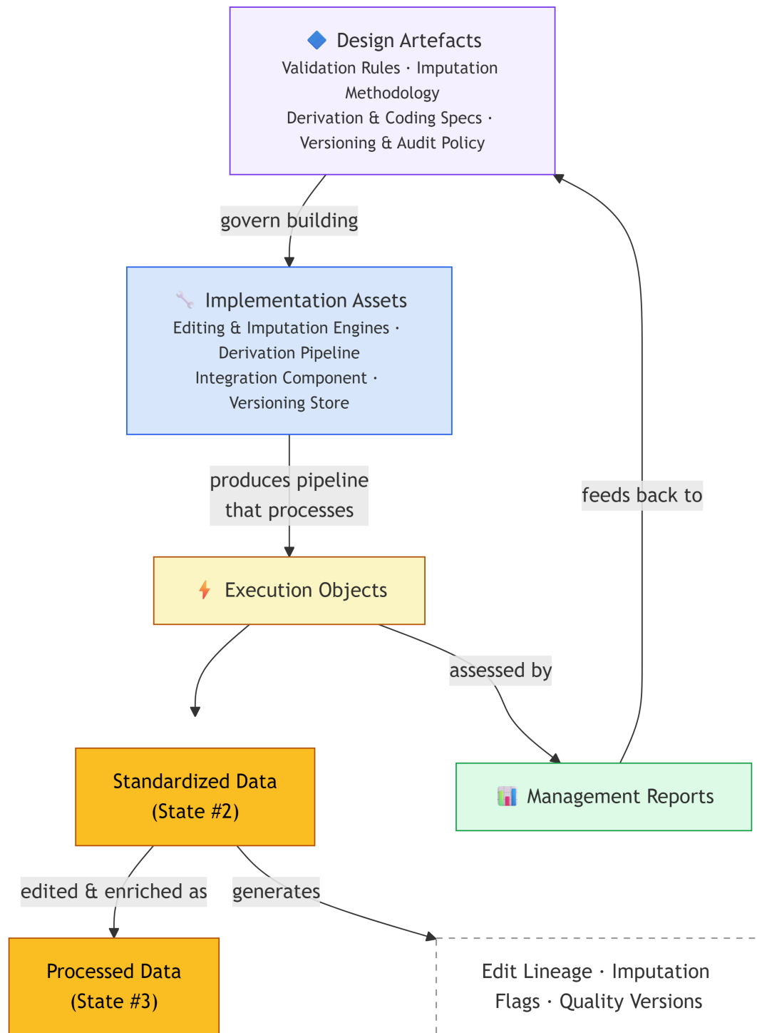
Figure 9: Business Object Lifecycle across all four process types. Design objects govern implementation, which produces the pipeline that edits and enriches execution objects, which are assessed by management objects, which feed back to design.
