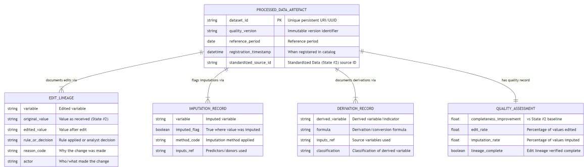
Figure 7: Processed Data Artefact Structure. Each processed quality version is linked to its edit lineage, imputation records, derivation records, and quality assessment, all traceable to the standardized source values.
